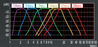
BPF Characteristics <IC-7610>
